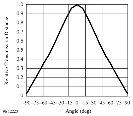
Figure 14. Directivity
